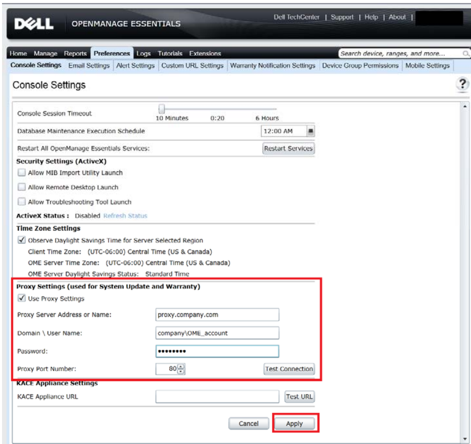
Figure 4 OME Proxy Settings
